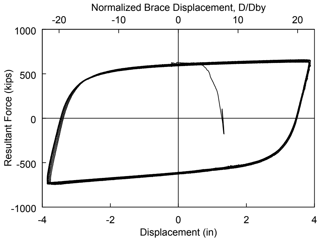
Fig. 5 Specimen 2D: Test 2 Brace Force versus Displacement Response
