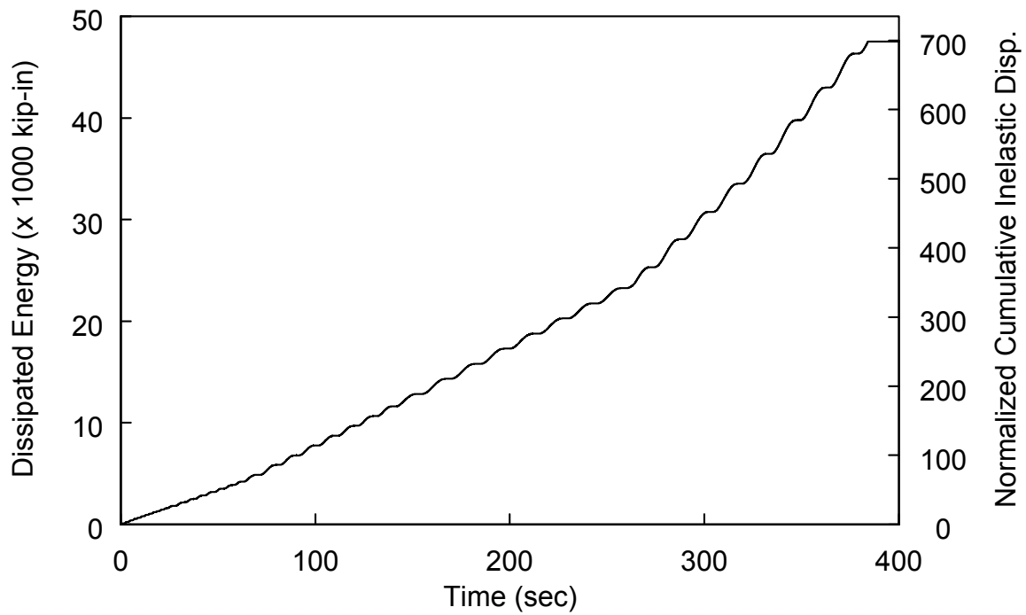
Fig. 3 Specimen 2D: Test 1 Dissipated Energy Time History
