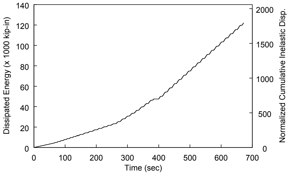
Fig. 9 Specimen 2D: Dissipated Energy Time History (Both Tests Combined)
