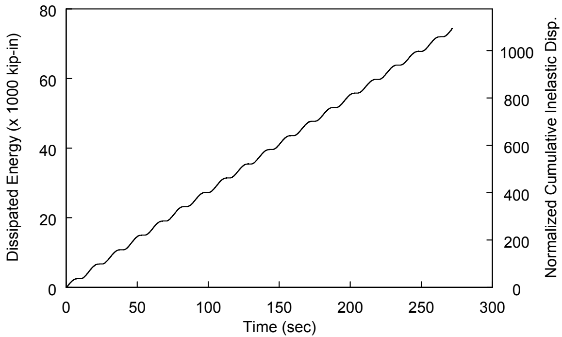
Fig. 6 Specimen 2D: Test 2 Dissipated Energy Time History
