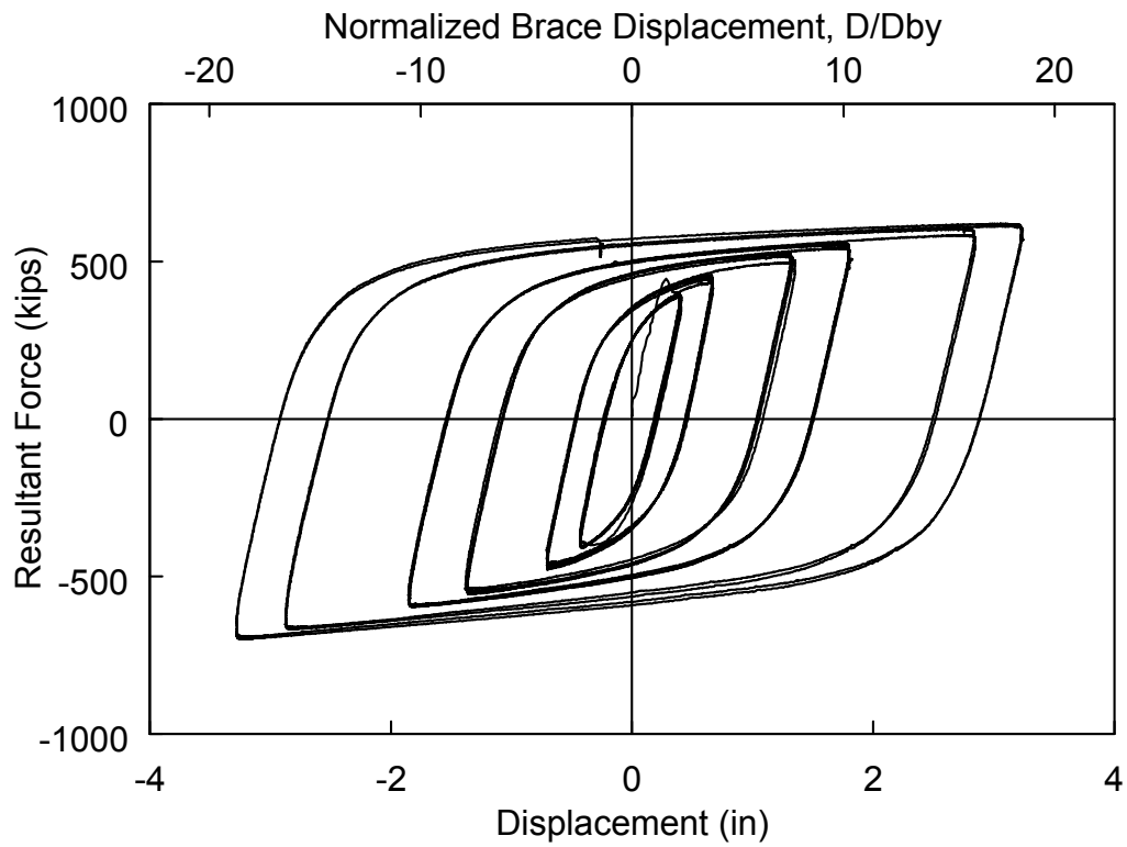
Fig. 2 Specimen 2D: Test 1 Brace Force versus Displacement Response
