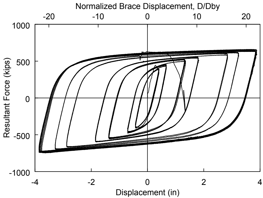
Fig. 8 Specimen 2D: Brace Force versus Displacement Response (Both Tests Combined)
