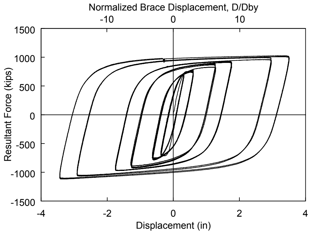
Fig. 2 Specimen 3D: Test 1 Brace Force versus Displacement Response
