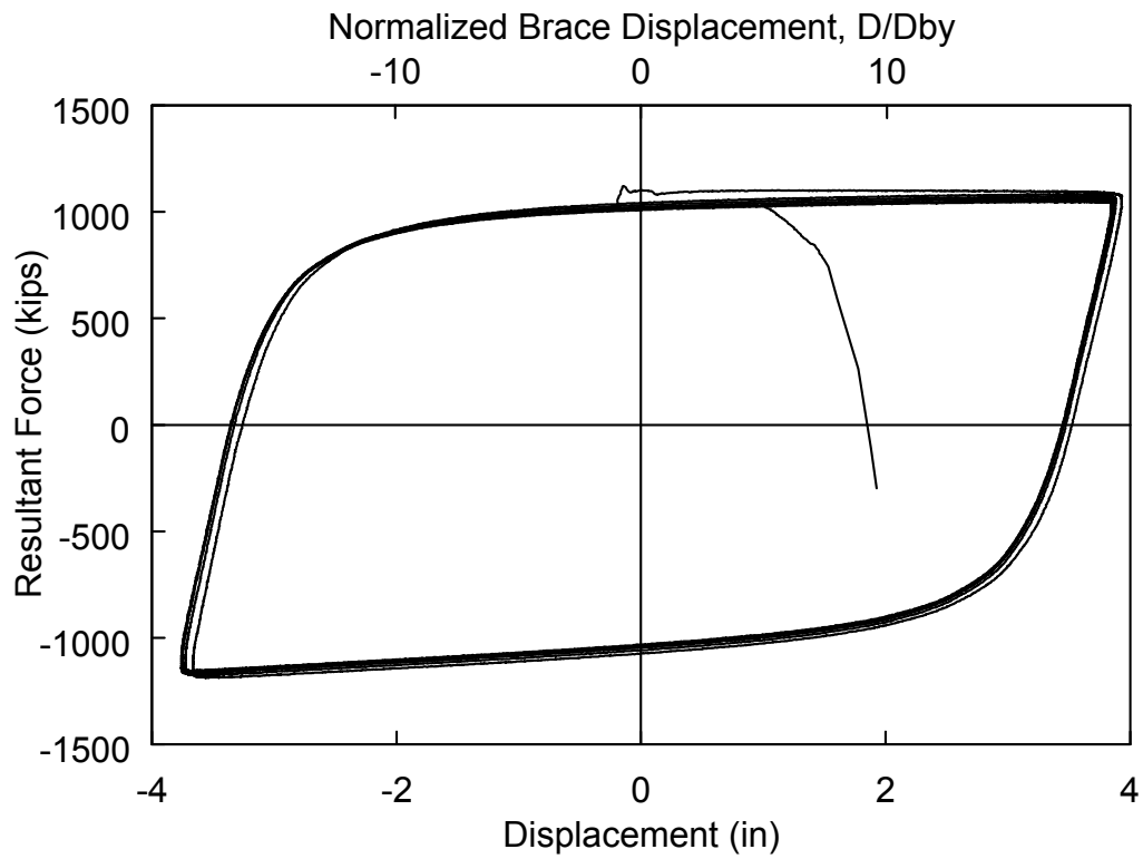
Fig. 5 Specimen 3D: Test 2 Brace Force versus Displacement Response
