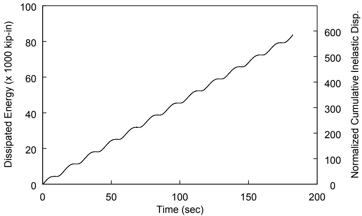
Fig. 6 Specimen 3D: Test 2 Dissipated Energy Time History
