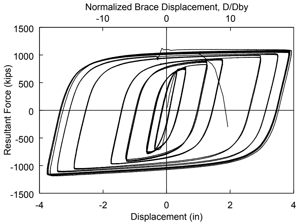
Fig. 8 Specimen 3D: Brace Force versus Displacement Response (Both Tests Combined)
