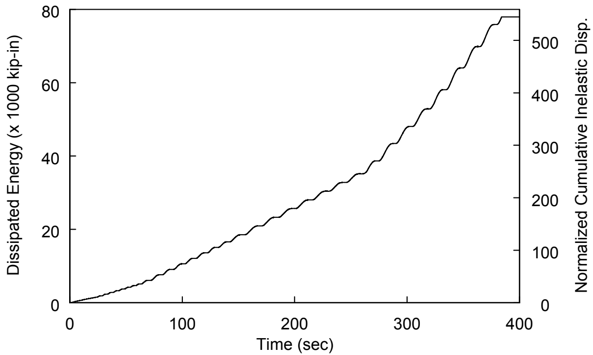
Fig. 3 Specimen 3D: Test 1 Dissipated Energy Time History
