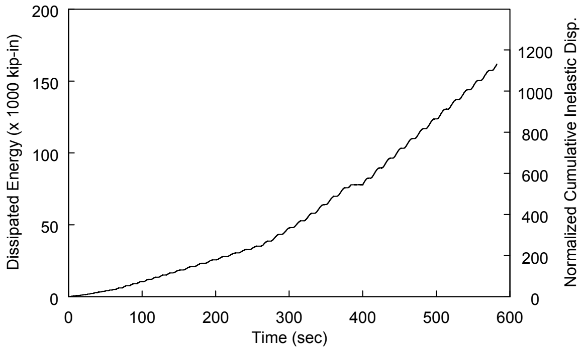
Fig. 9 Specimen 3D: Dissipated Energy Time History (Both Tests Combined)
